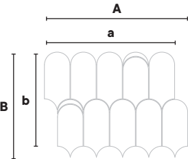
A 41,2 cm / 16" a 37,469 cm / 15" B 30,3 cm / 12" b 27,119 cm / 11"
